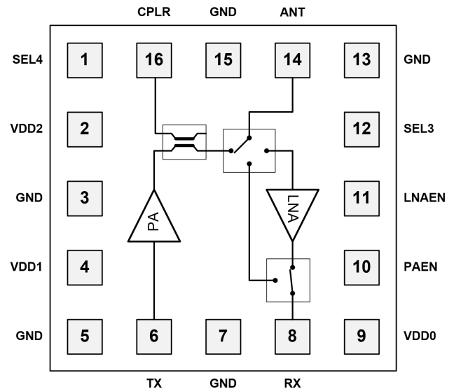
16-pin LGA 2x2 mm
